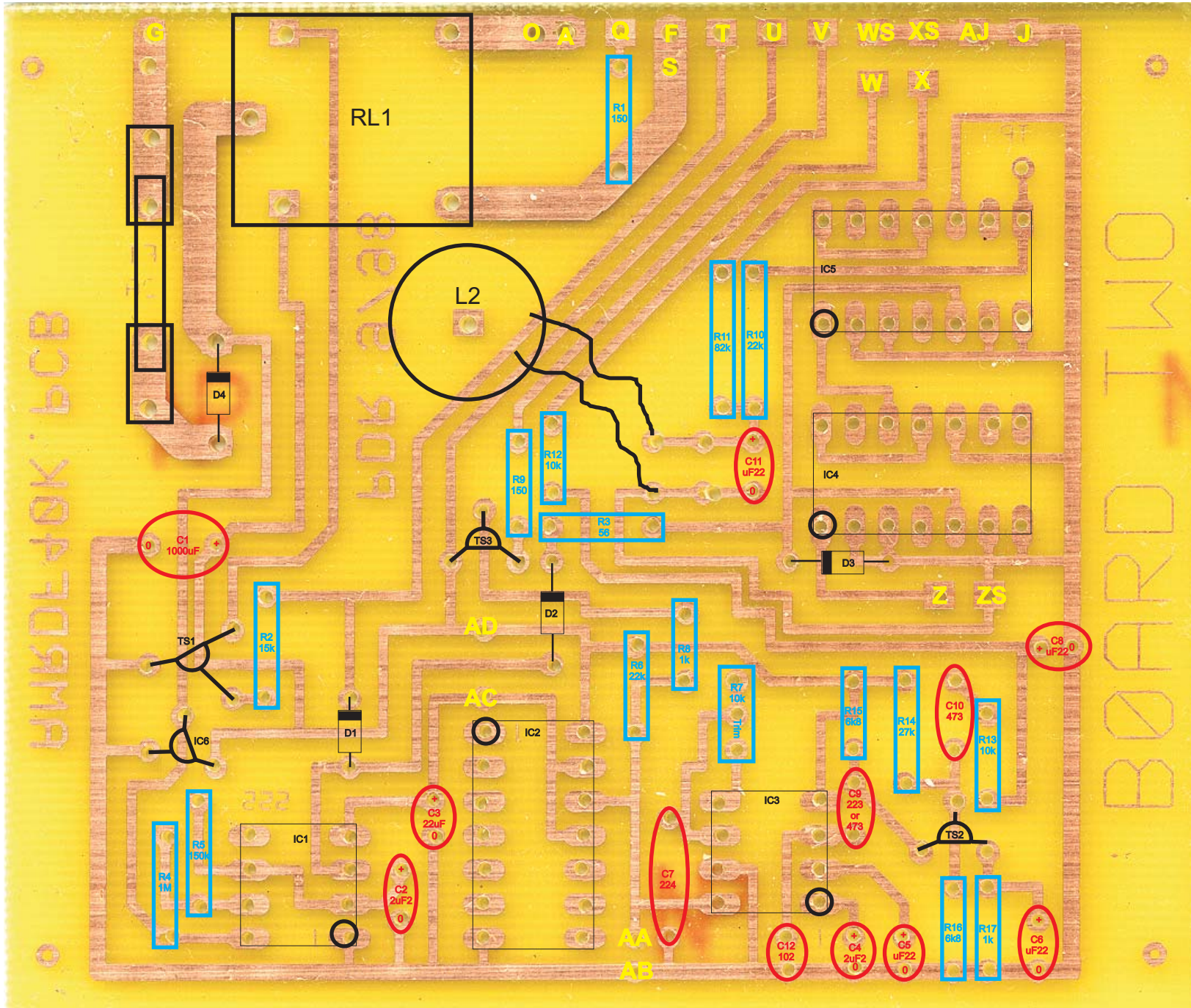
BOARD 2 - COMPONENT SIDE VIEW
